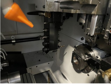
Main spindle
